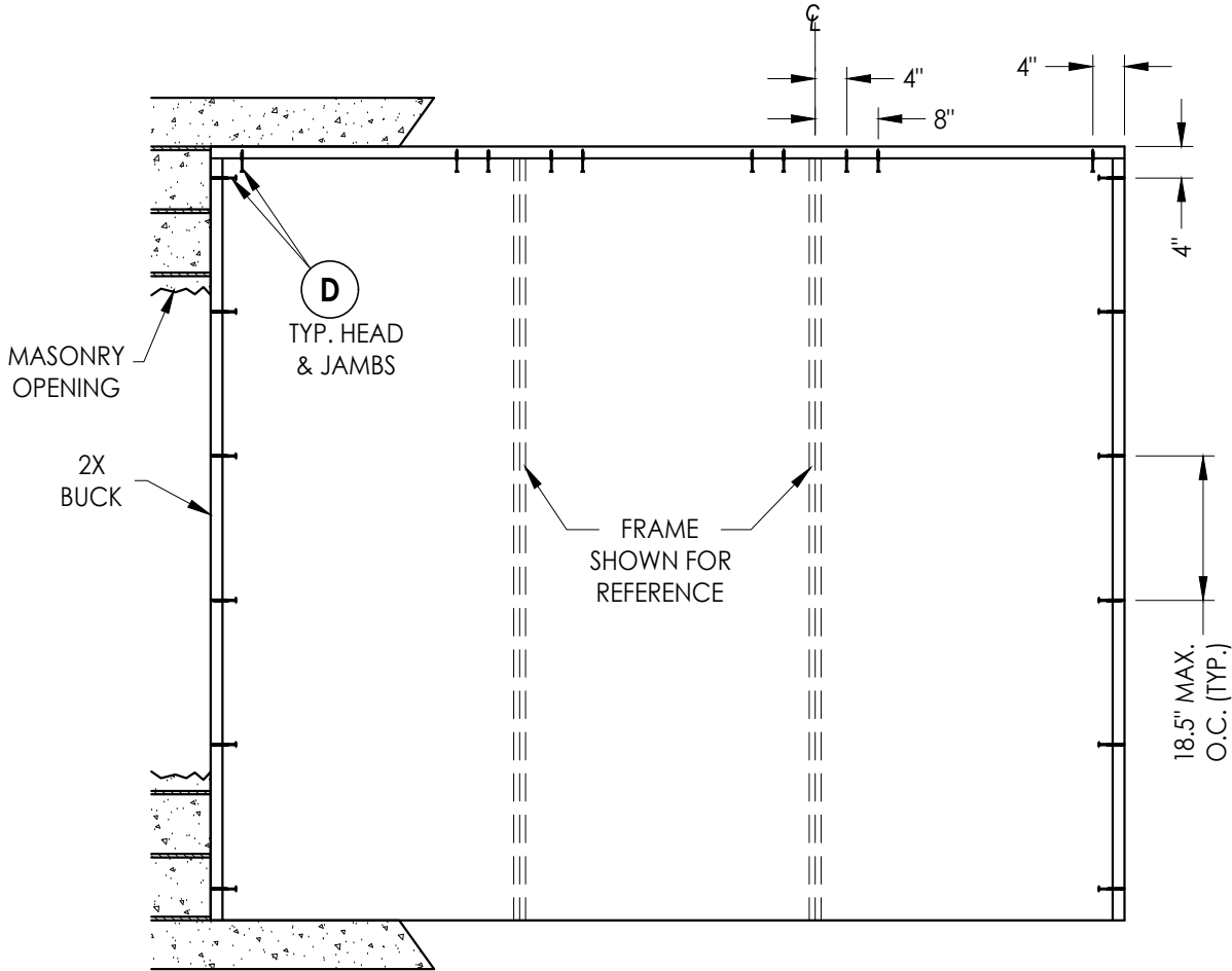
BUCK ANCHORING
