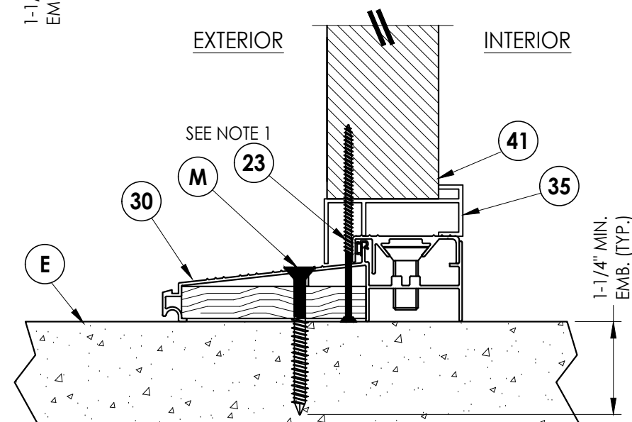
5 VERTICAL CROSS SECTION
